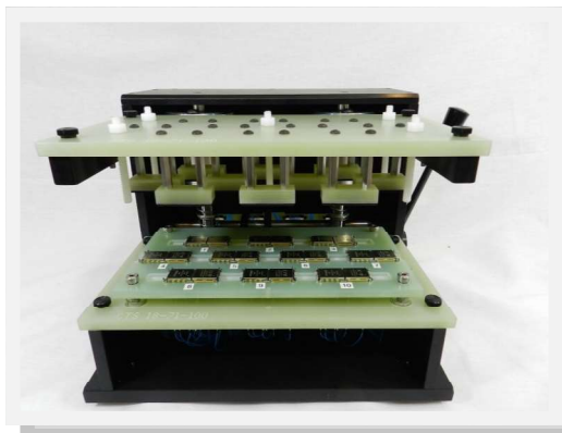
1012 Reusable Mechanical Press testing 10 non-panelized UUTs simultaneously.
